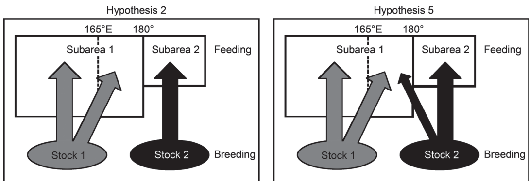
Fig. 2. The two hypotheses considered in the Implementation Simulation Trials (see text).
