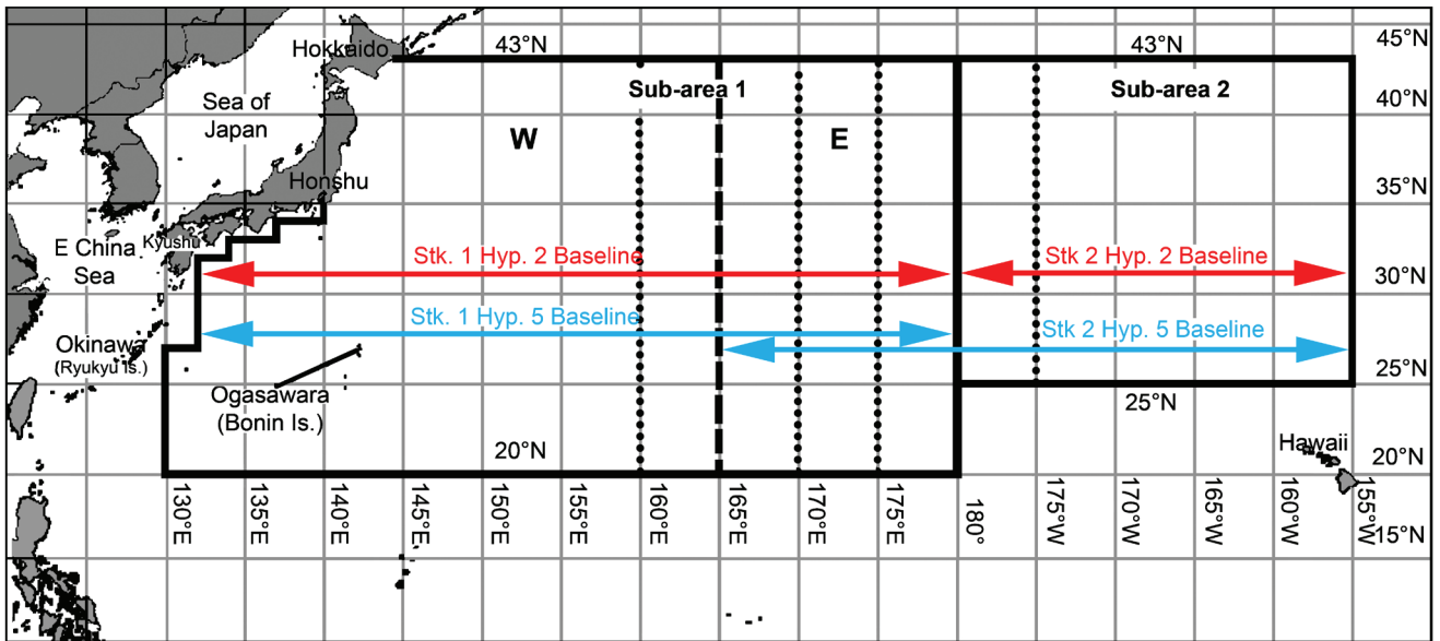
Fig. 1. Map of the western North Pacific showing the sub-areas defined for the western North Pacific Bryde’s whales Implementation Review . The ranges of the stocks for Hypotheses 2 and 5 (baselines) are also shown. The boundary between the sub-areas 1W and 1E at 165°E, indicated by a dashed line, is a management boundary (used by the RMP). The dotted lines at 160°E, 170°E, 175°E and 175°W denote the boundaries between the ‘Component-areas’ and are used for trials in which the true boundary between the stocks differs from the boundary on which the RMP is based. The staggered border to the south of Japan is used to ensure that no catches of the inshore form of Bryde’s whales are included in these trials.
